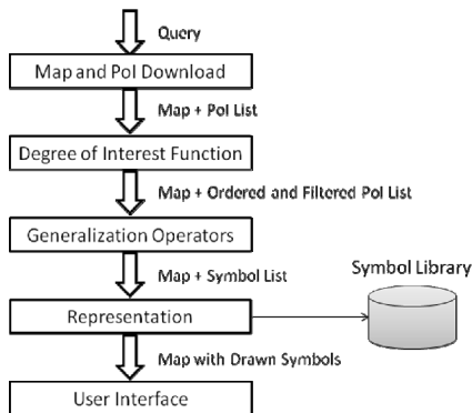
Figure 6: MoViSys execution flow.
