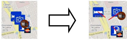
Figure 5: Displacement Operator.
